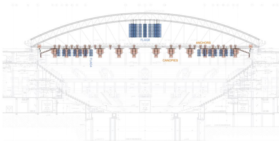
ARENA - JERUSALEM 1:200 MAY 2023 ACOUSTIC PANELS SECTION
